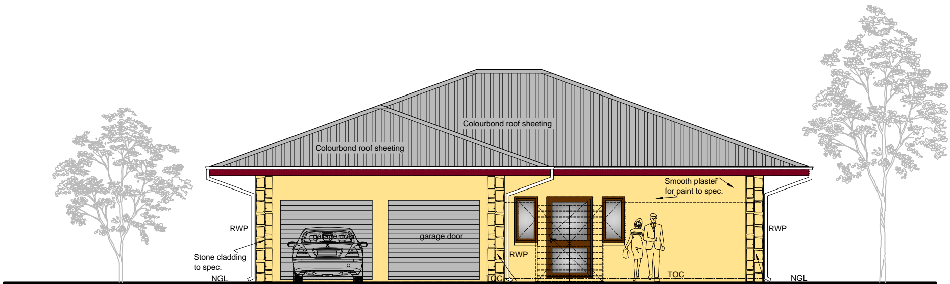
ELEVATION 1-1
